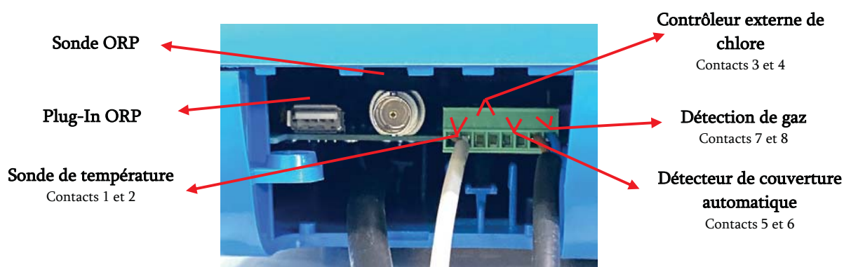
Figure 6 - Connexions internes
